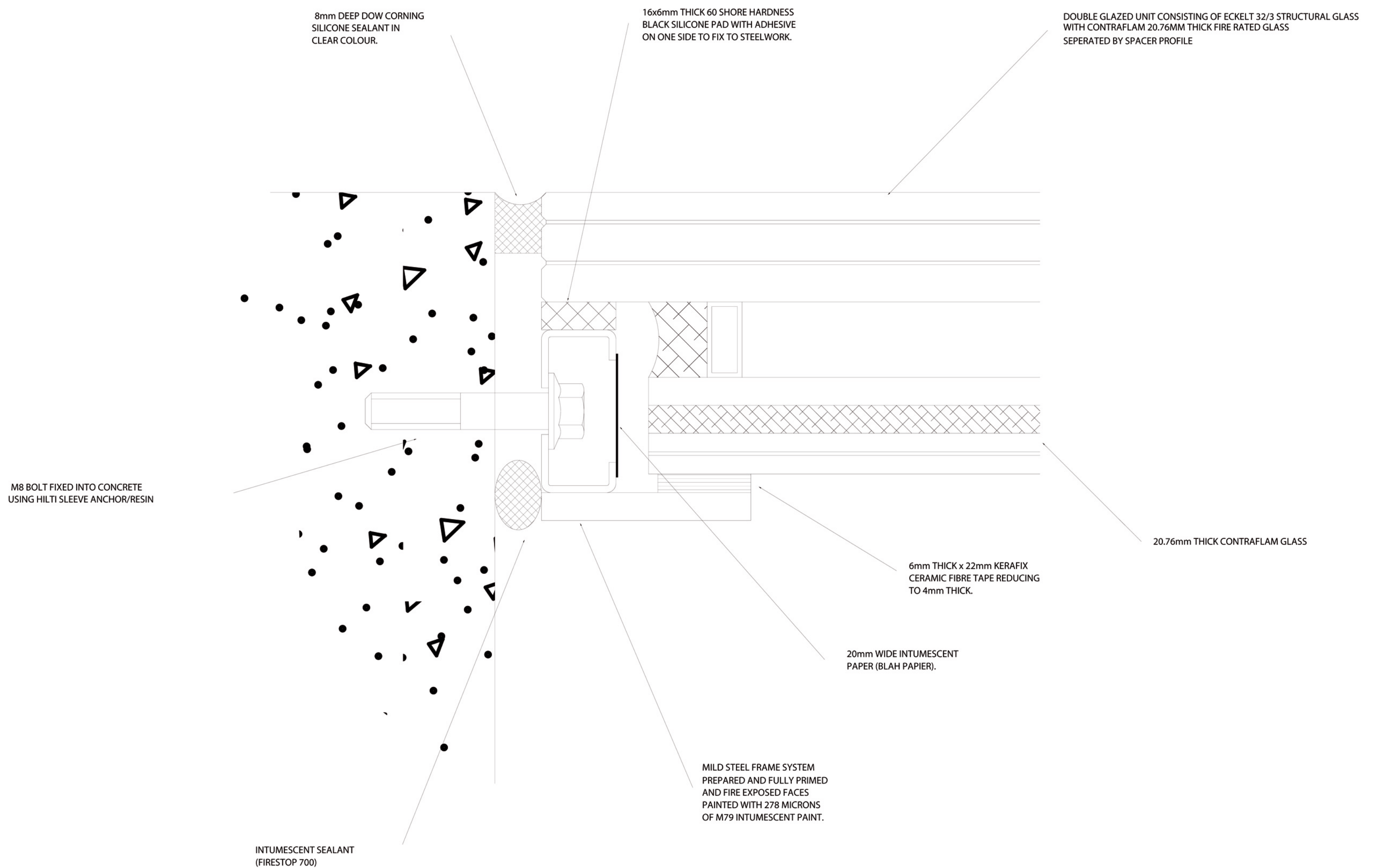
Liteflam Typical Edge Detail
